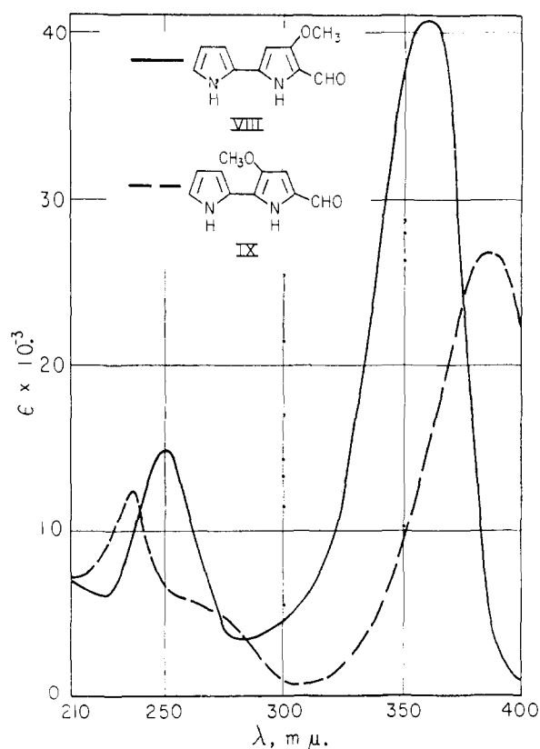
Fig. 1.—Ultraviolet absorption spectra in methanol of 4-methoxy-2,2'-bipyrrole-5-carboxaldehyde (VIII) (—) and 3-methoxy-2,2'-bipyrrole-5-carboxaldehyde (IX) (---).
